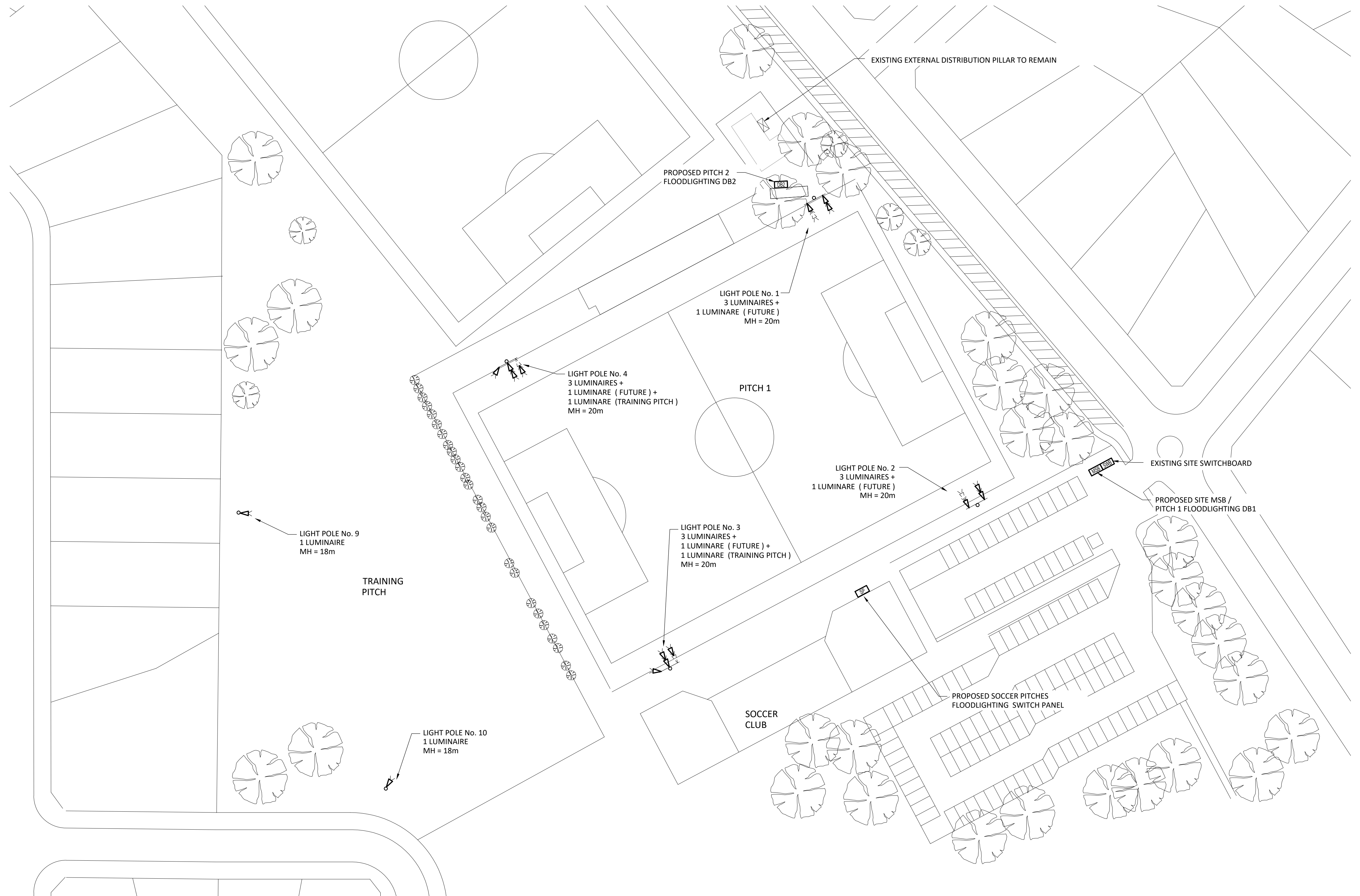
PROPOSED FLOODLIGHTING LAYOUT - SOCCER PITCH 1 & TRAINING PITCH SCALE 1:500
